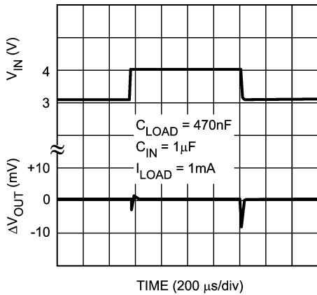
Line Transient
